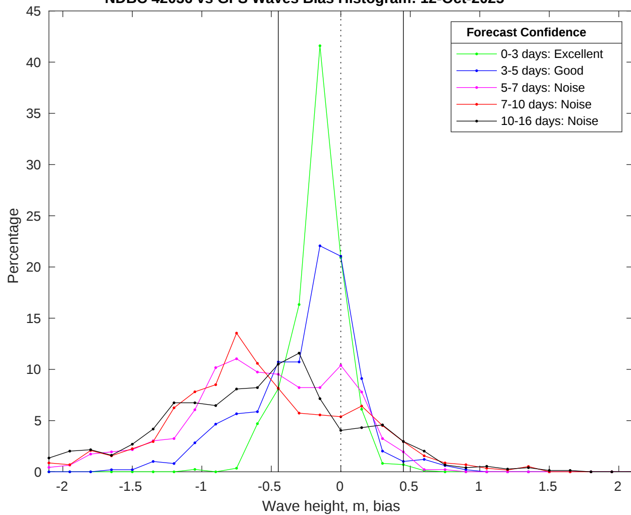
NDBC 42036 vs GFS Waves Bias Histogram: 12-Oct-2025
