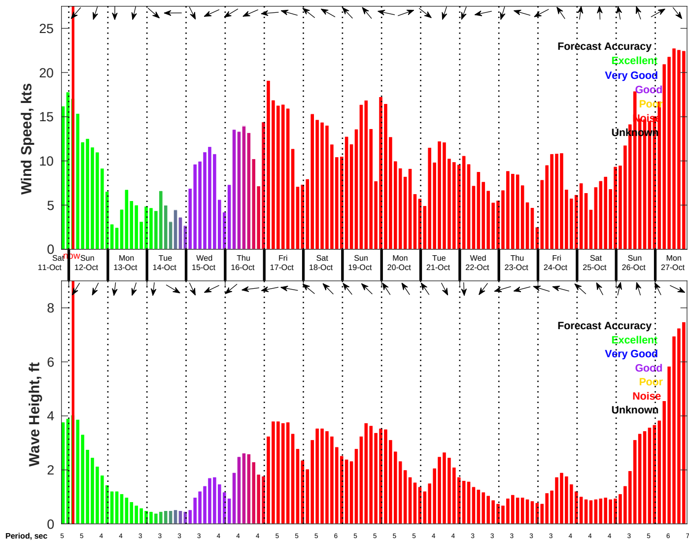
Wind & Wave Forecast for NDBC 42036 from 11-Oct-2025 19:00:00 to 27-Oct-2025 19:00:00
