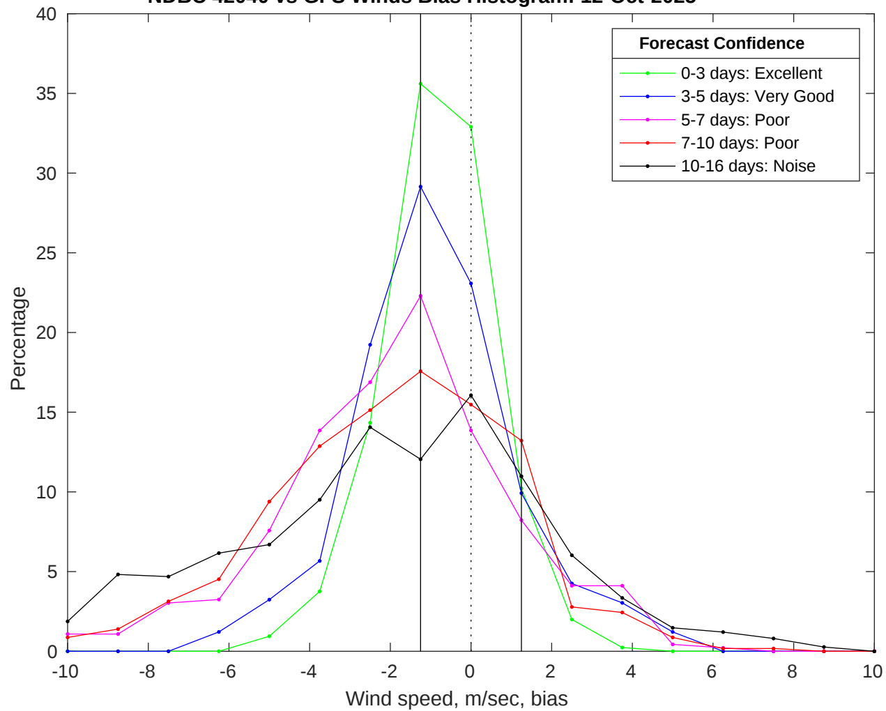
NDBC 42040 vs GFS Winds Bias Histogram: 12-Oct-2025
