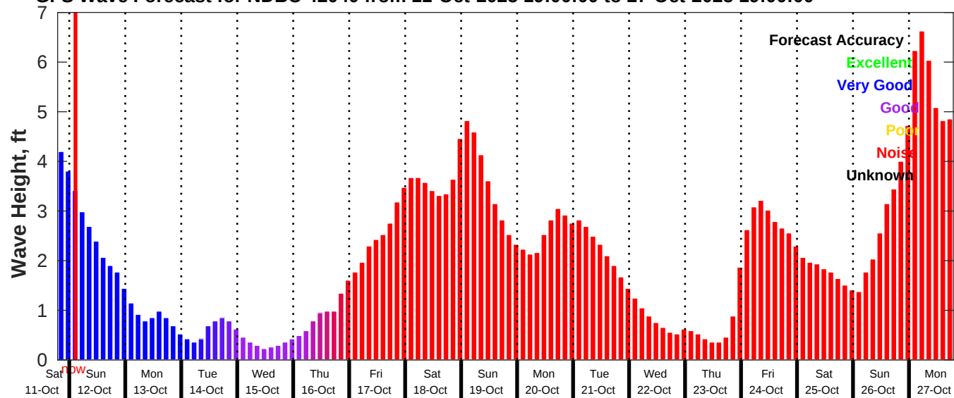
GFS Wave Forecast for NDBC 42040 from 11-Oct-2025 19:00:00 to 27-Oct-2025 19:00:00
