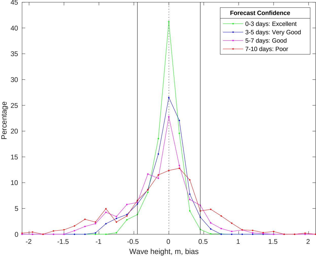
NDBC 44008 vs CMEMS Waves Bias Histogram: 12-Oct-2025
