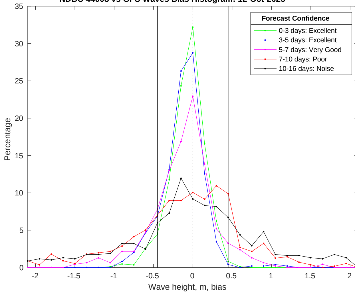
NDBC 44008 vs GFS Waves Bias Histogram: 12-Oct-2025
