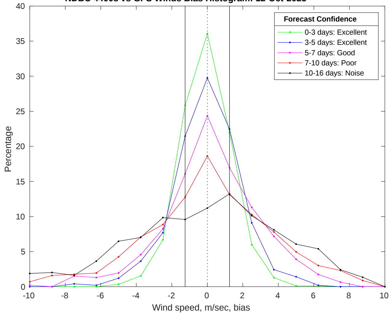
NDBC 44008 vs GFS Winds Bias Histogram: 12-Oct-2025
