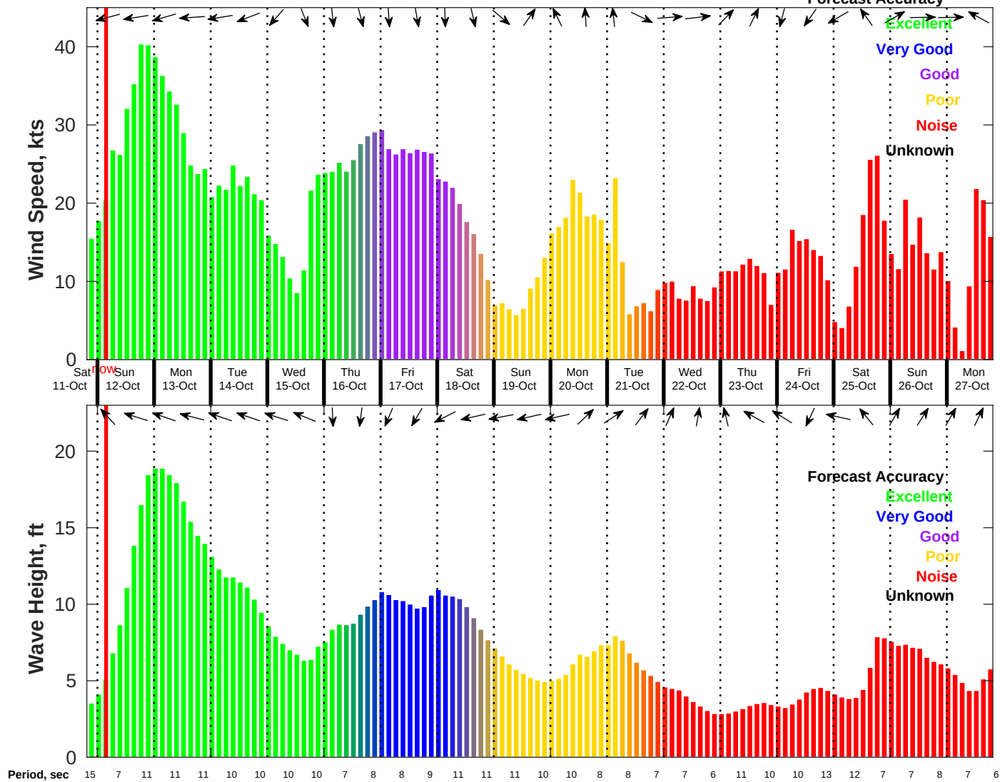
Wind & Wave Forecast for NDBC 44008 from 11-Oct-2025 20:00:00 to 27-Oct-2025 20:00:00
