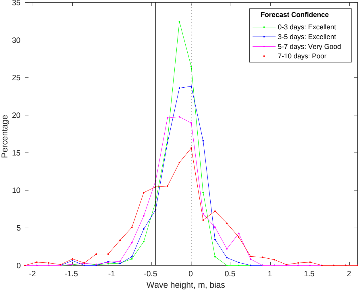
NDBC 46011 vs CMEMS Waves Bias Histogram: 12-Oct-2025
