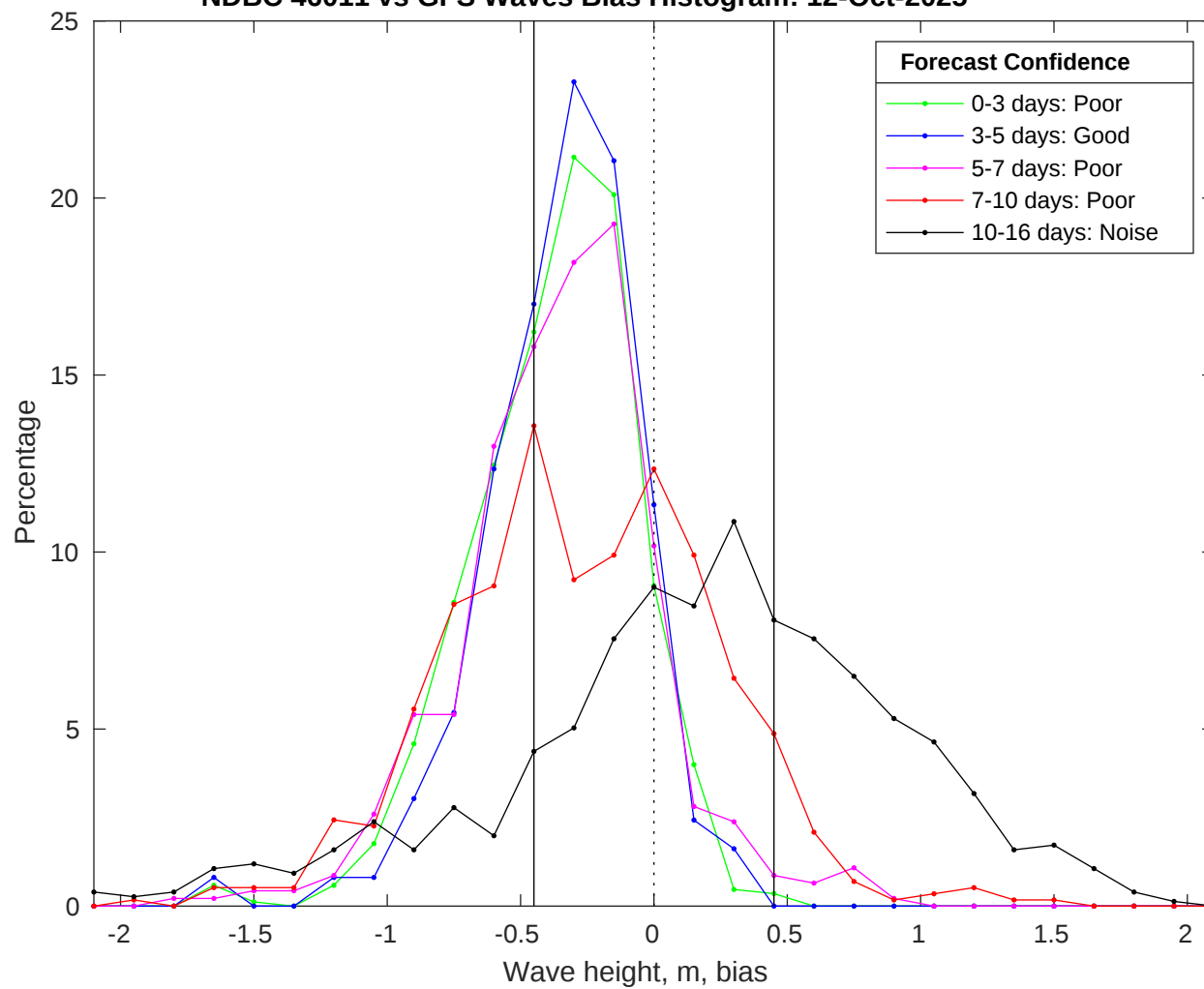
NDBC 46011 vs GFS Waves Bias Histogram: 12-Oct-2025
