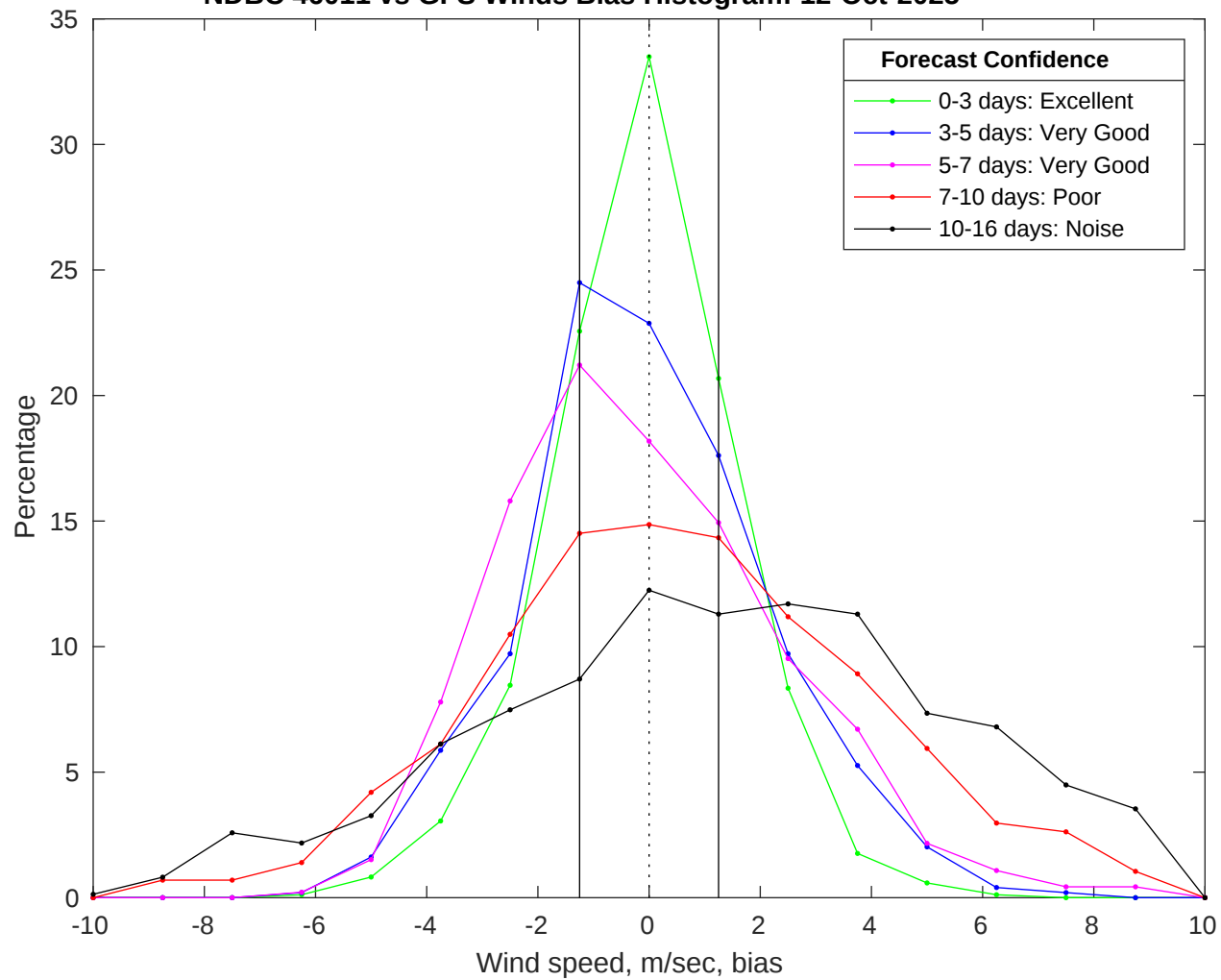
NDBC 46011 vs GFS Winds Bias Histogram: 12-Oct-2025
