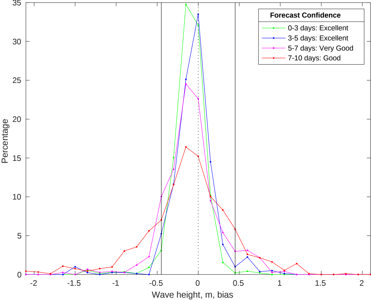
NDBC 46028 vs CMEMS Waves Bias Histogram: 12-Oct-2025
