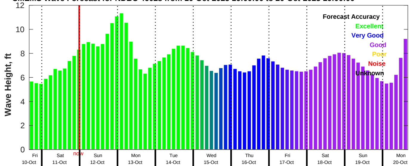
CMEMS Wave Forecast for NDBC 46028 from 10-Oct-2025 16:00:00 to 20-Oct-2025 16:00:00
