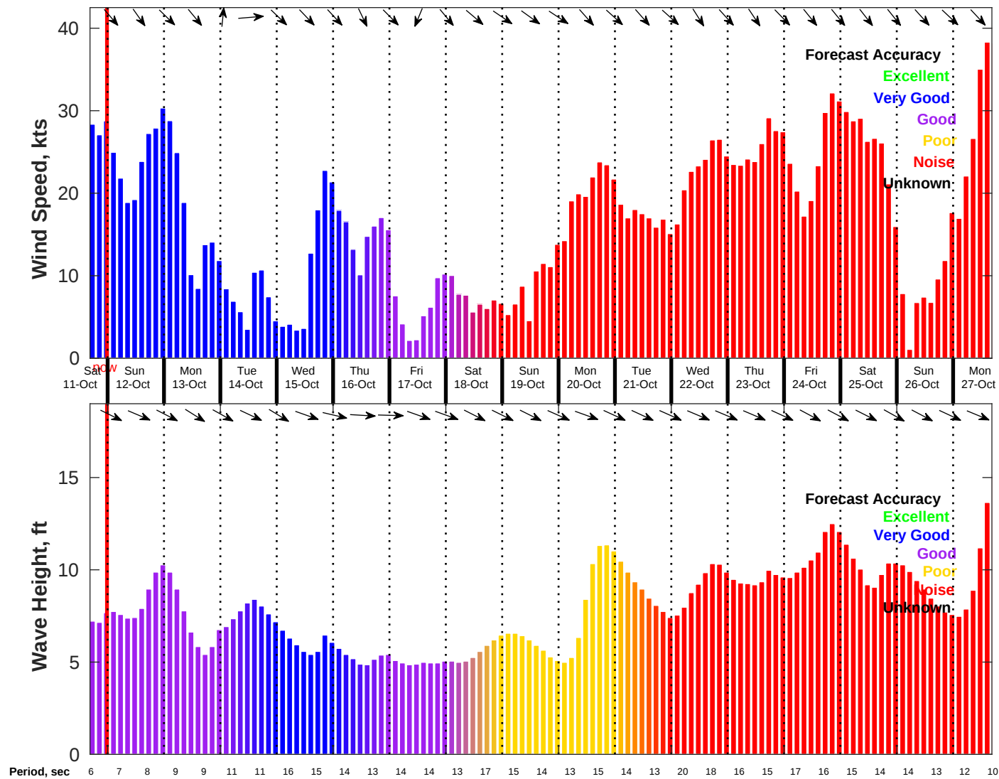
Wind & Wave Forecast for NDBC 46028 from 11-Oct-2025 16:00:00 to 27-Oct-2025 16:00:00
