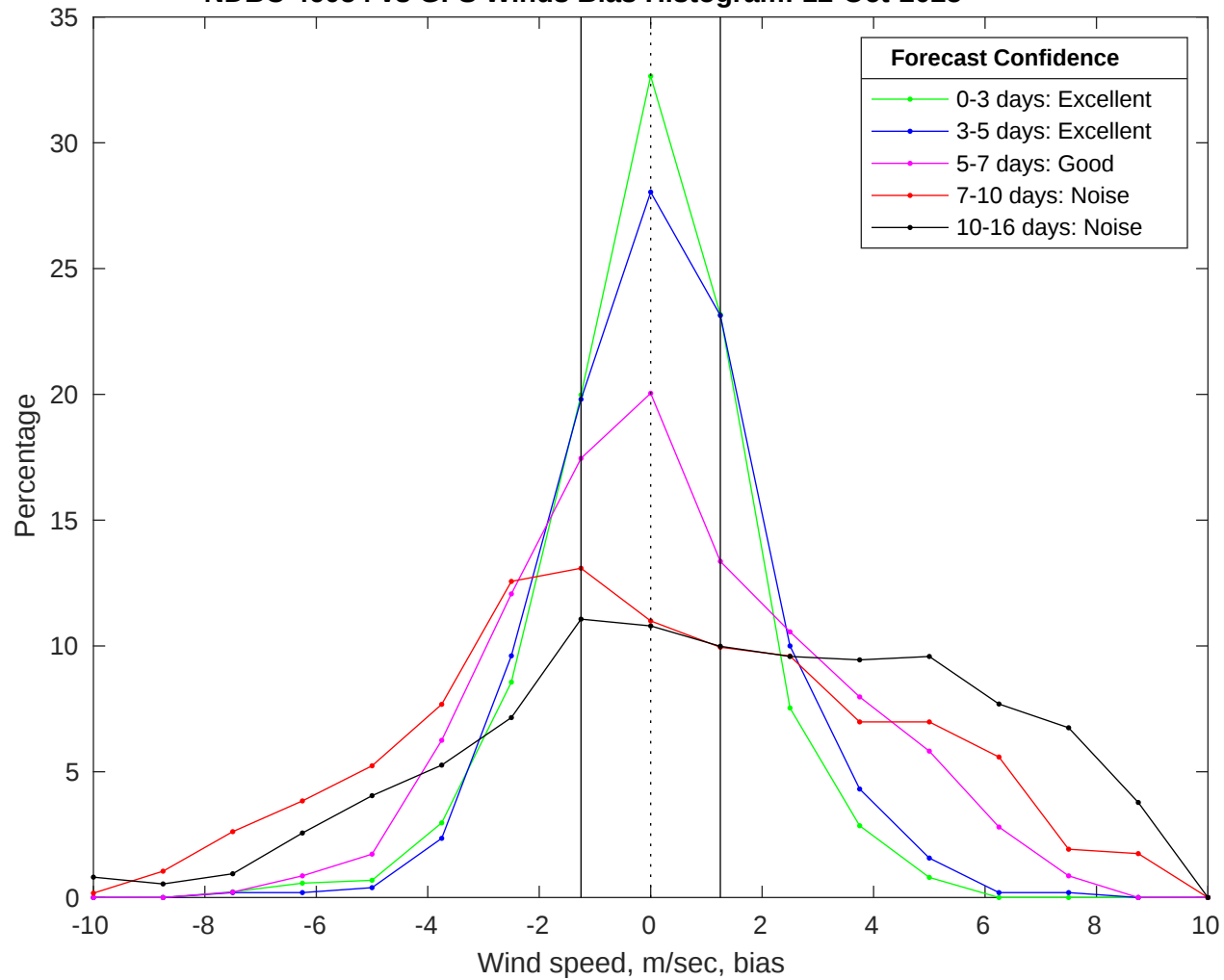
NDBC 46054 vs GFS Winds Bias Histogram: 12-Oct-2025
