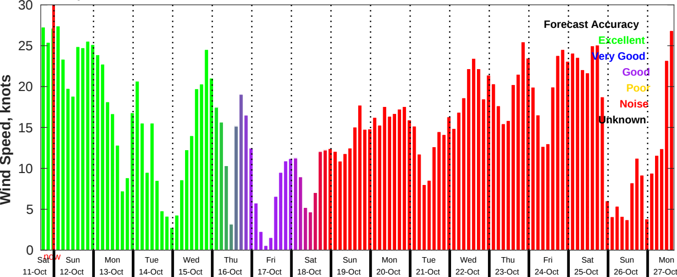
GFS Wind Speed Forecast for NDBC 46054 from 11-Oct-2025 16:00:00 to 27-Oct-2025 16:00:00
