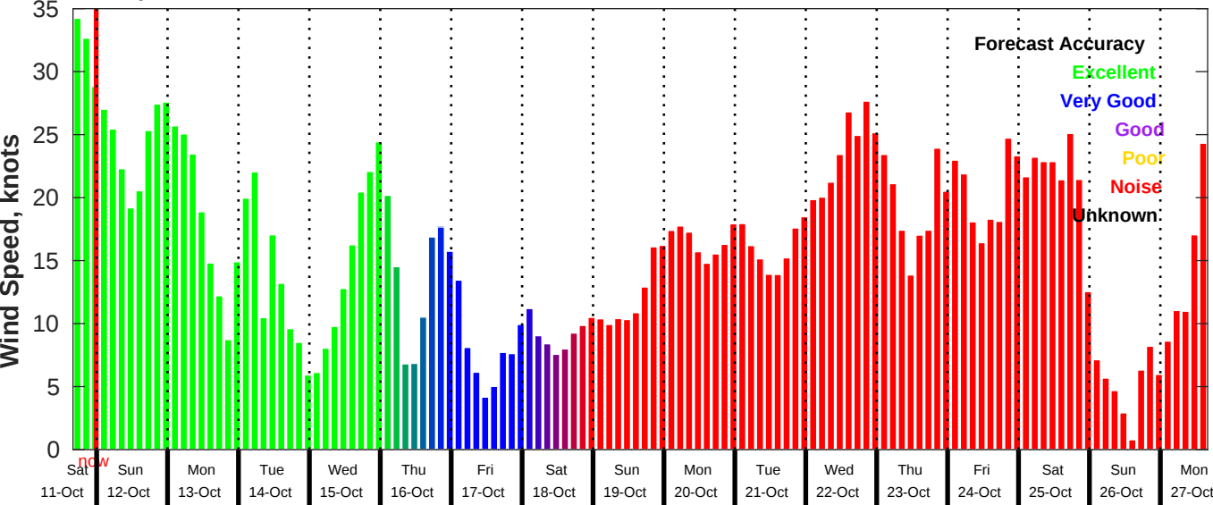
GFS Wind Speed Forecast for NDBC 46069 from 11-Oct-2025 16:00:00 to 27-Oct-2025 16:00:00
