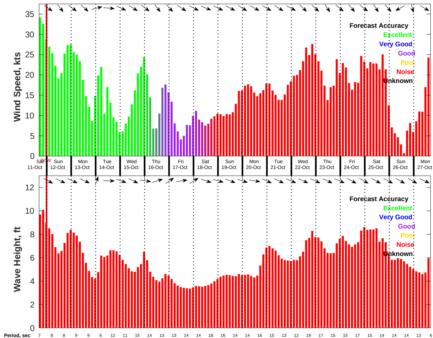
Wind & Wave Forecast for NDBC 46069 from 11-Oct-2025 16:00:00 to 27-Oct-2025 16:00:00
