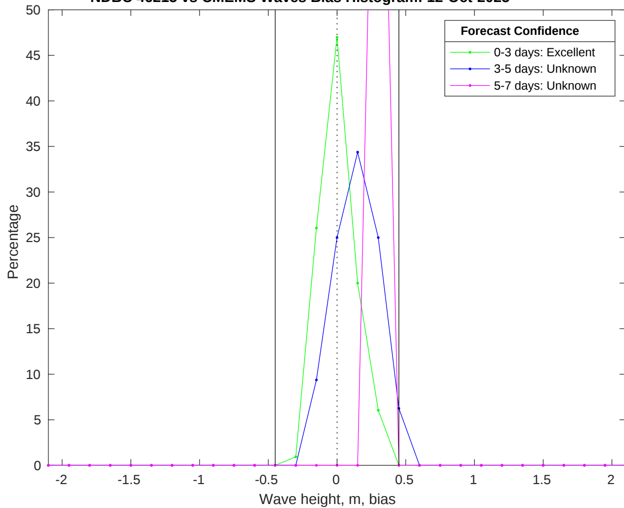
NDBC 46215 vs CMEMS Waves Bias Histogram: 12-Oct-2025
