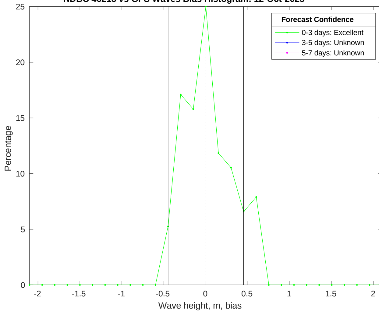
NDBC 46215 vs GFS Waves Bias Histogram: 12-Oct-2025
