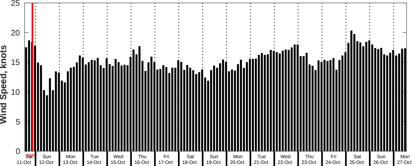
GFS Wind Speed Forecast for NDBC 51209 from 11-Oct-2025 13:00:00 to 27-Oct-2025 13:00:00
