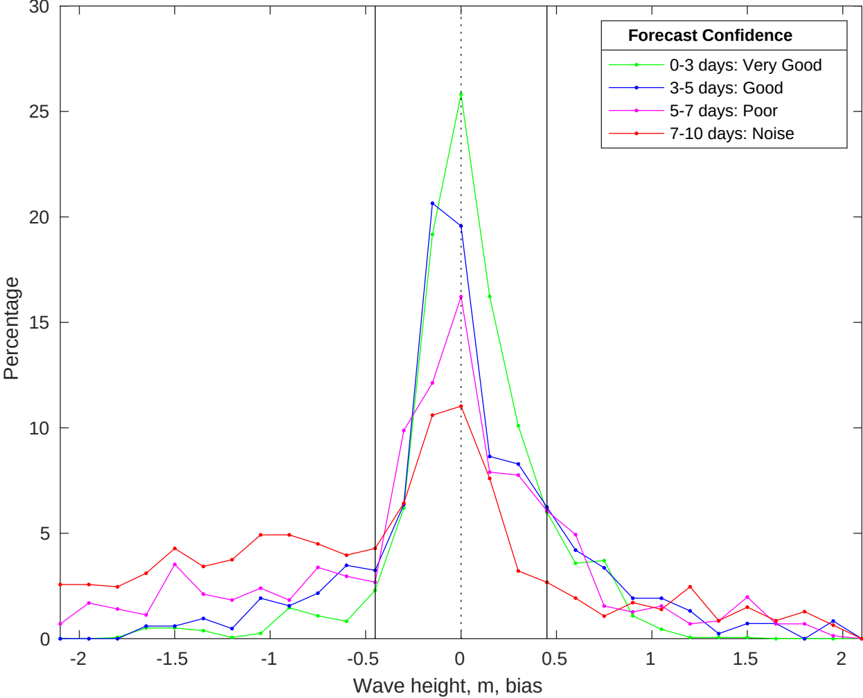
NDBC 41004 vs CMEMS Waves Bias Histogram: 13-Oct-2025
