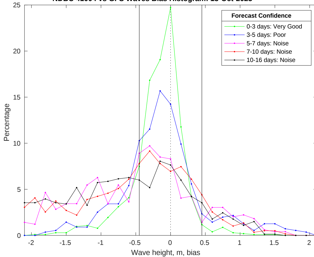
NDBC 41004 vs GFS Waves Bias Histogram: 13-Oct-2025
