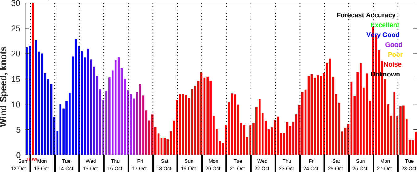
GFS Wind Speed Forecast for NDBC 41004 from 12-Oct-2025 19:00:00 to 28-Oct-2025 19:00:00
