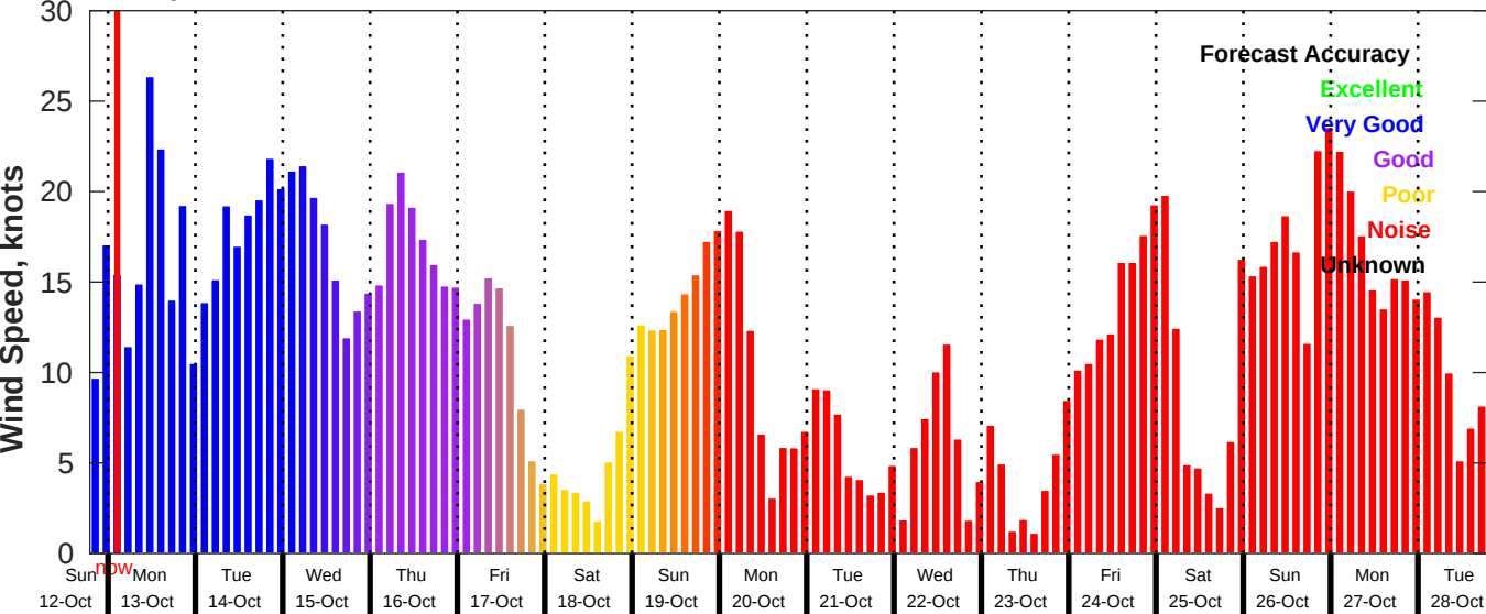
GFS Wind Speed Forecast for NDBC 41013 from 12-Oct-2025 19:00:00 to 28-Oct-2025 19:00:00
