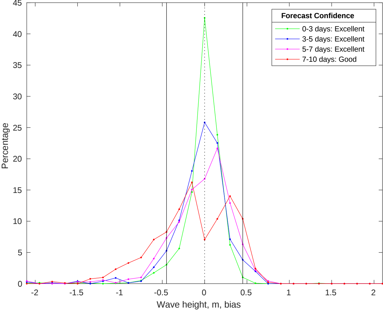
NDBC 41040 vs CMEMS Waves Bias Histogram: 13-Oct-2025
