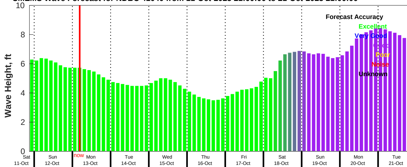
CMEMS Wave Forecast for NDBC 41040 from 11-Oct-2025 21:00:00 to 21-Oct-2025 21:00:00
