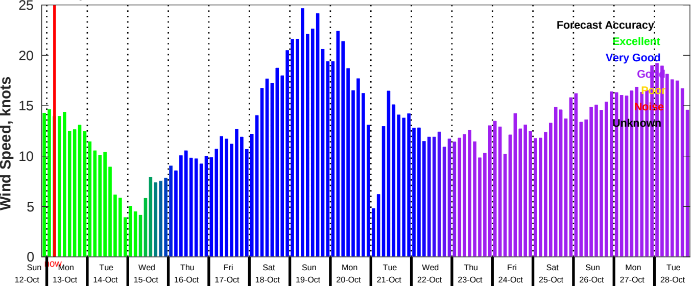
GFS Wind Speed Forecast for NDBC 41040 from 12-Oct-2025 21:00:00 to 28-Oct-2025 21:00:00
