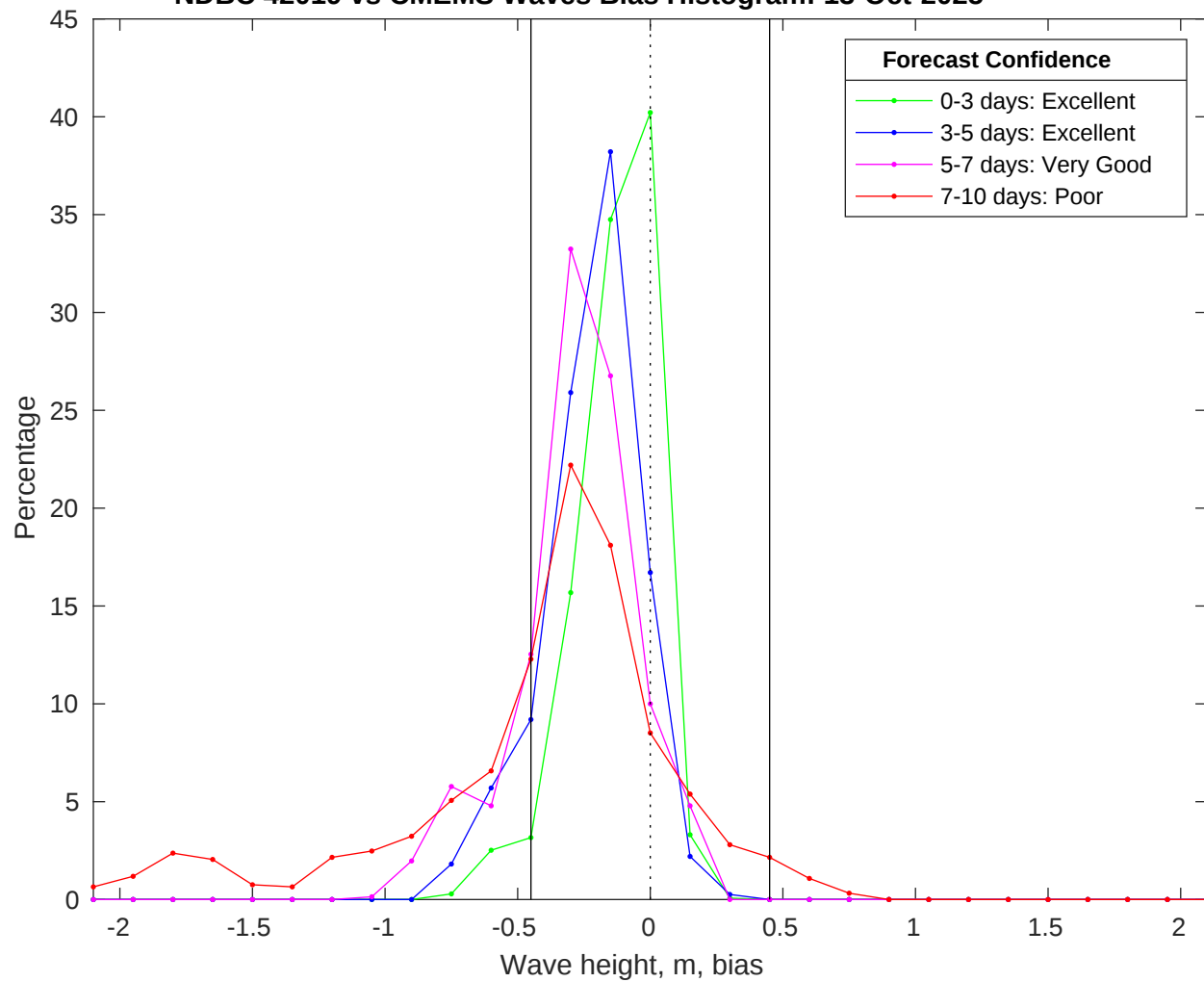
NDBC 42019 vs CMEMS Waves Bias Histogram: 13-Oct-2025
