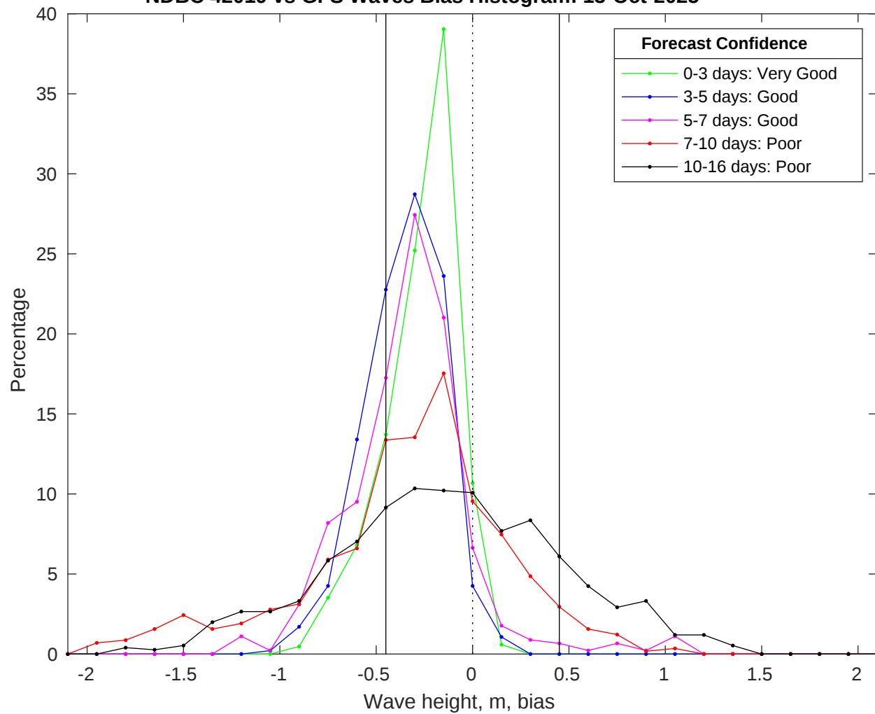
NDBC 42019 vs GFS Waves Bias Histogram: 13-Oct-2025
