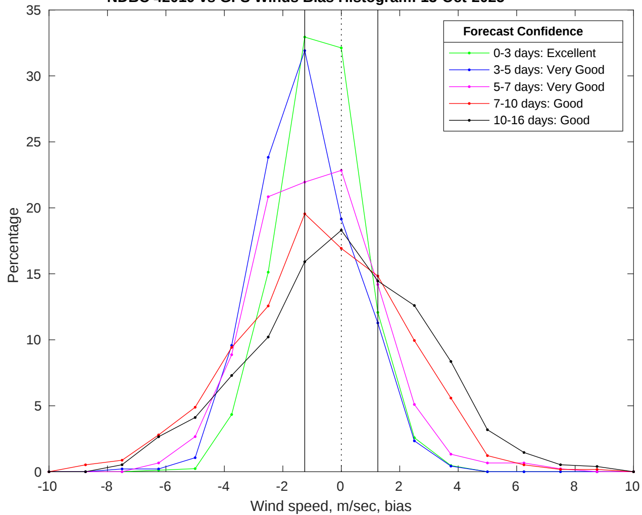
NDBC 42019 vs GFS Winds Bias Histogram: 13-Oct-2025
