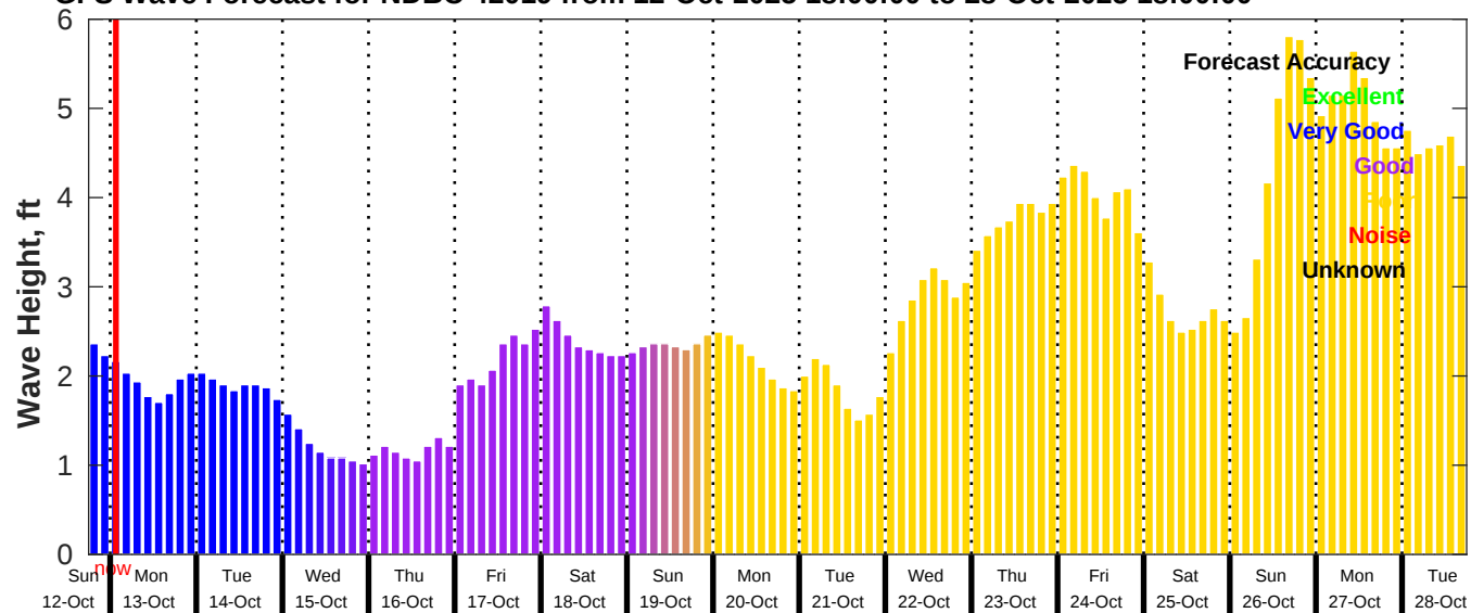
GFS Wave Forecast for NDBC 42019 from 12-Oct-2025 18:00:00 to 28-Oct-2025 18:00:00
