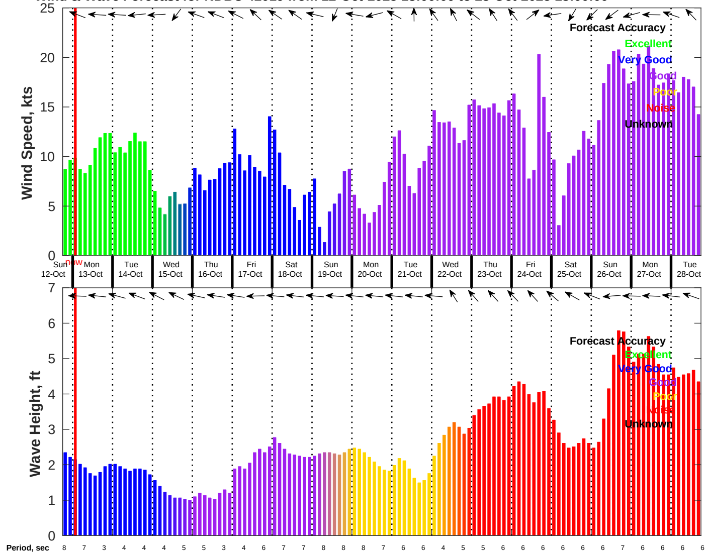
Wind & Wave Forecast for NDBC 42019 from 12-Oct-2025 18:00:00 to 28-Oct-2025 18:00:00
