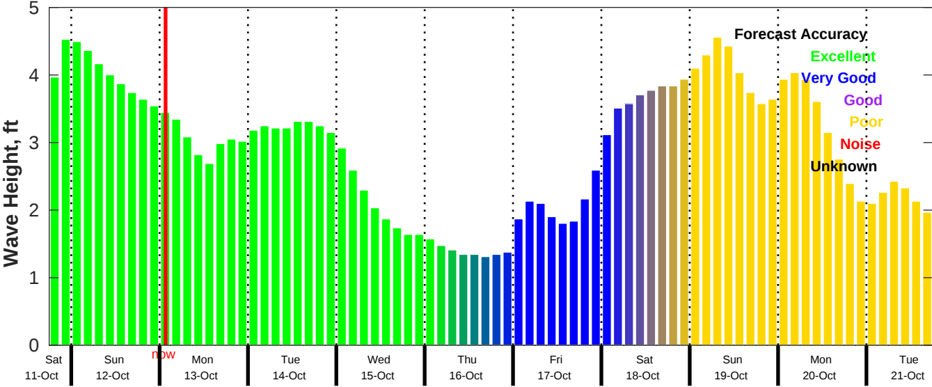
CMEMS Wave Forecast for NDBC 42020 from 11-Oct-2025 18:00:00 to 21-Oct-2025 18:00:00
