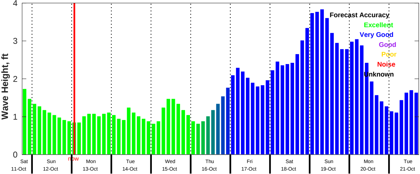
CMEMS Wave Forecast for NDBC 42035 from 11-Oct-2025 18:00:00 to 21-Oct-2025 18:00:00
