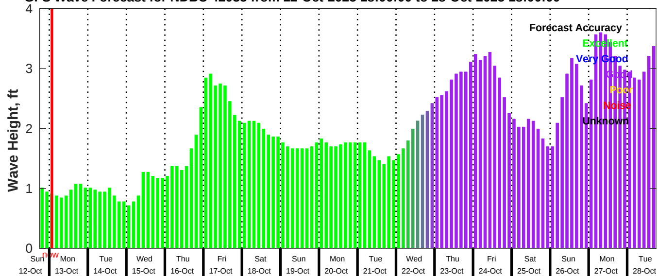
GFS Wave Forecast for NDBC 42035 from 12-Oct-2025 18:00:00 to 28-Oct-2025 18:00:00
