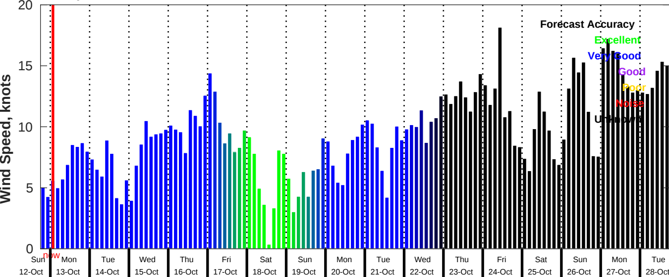
GFS Wind Speed Forecast for NDBC 42035 from 12-Oct-2025 18:00:00 to 28-Oct-2025 18:00:00
