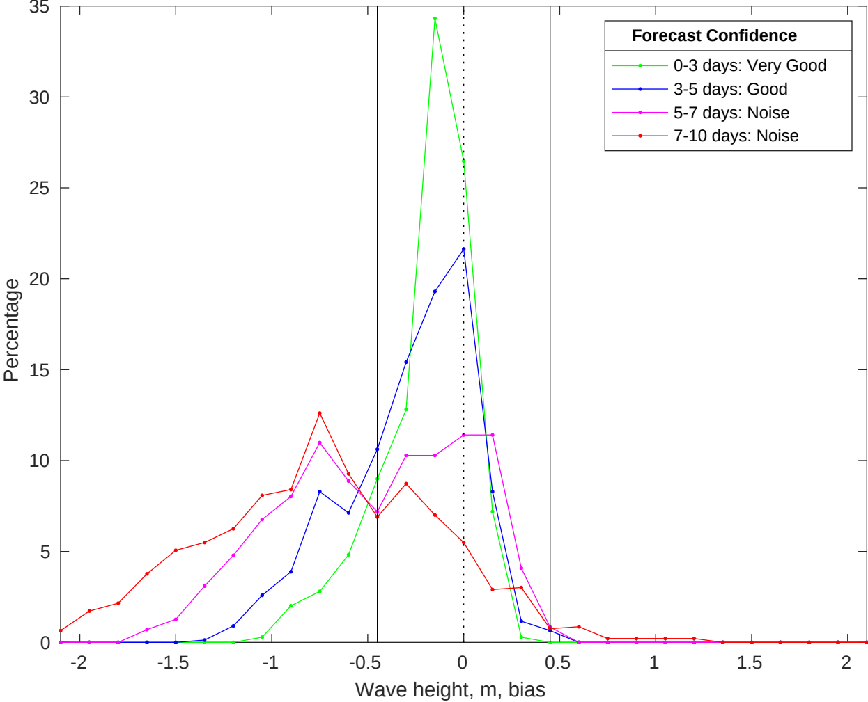
NDBC 42036 vs CMEMS Waves Bias Histogram: 13-Oct-2025
