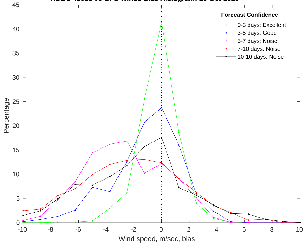
NDBC 42036 vs GFS Winds Bias Histogram: 13-Oct-2025
