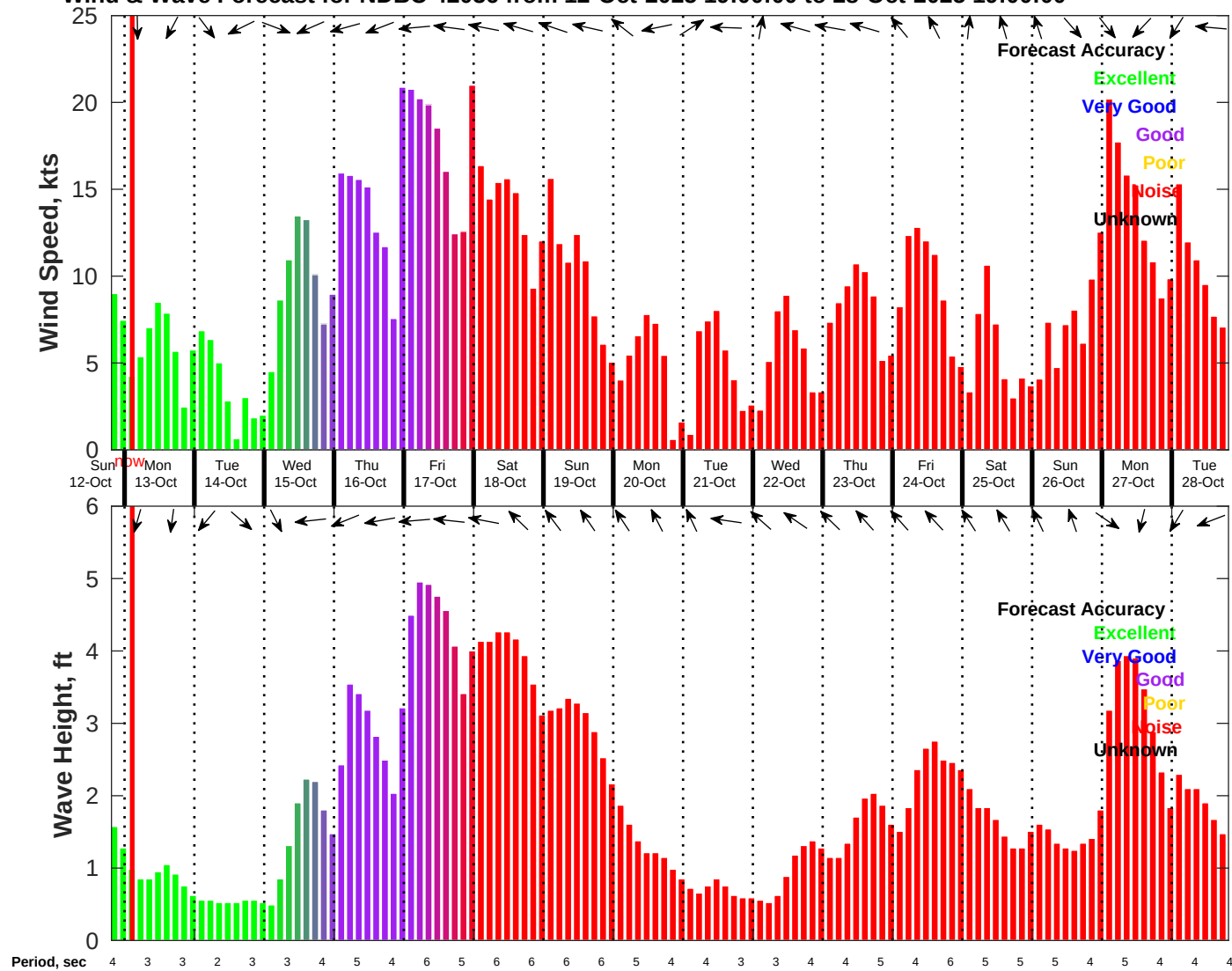
Wind & Wave Forecast for NDBC 42036 from 12-Oct-2025 19:00:00 to 28-Oct-2025 19:00:00
