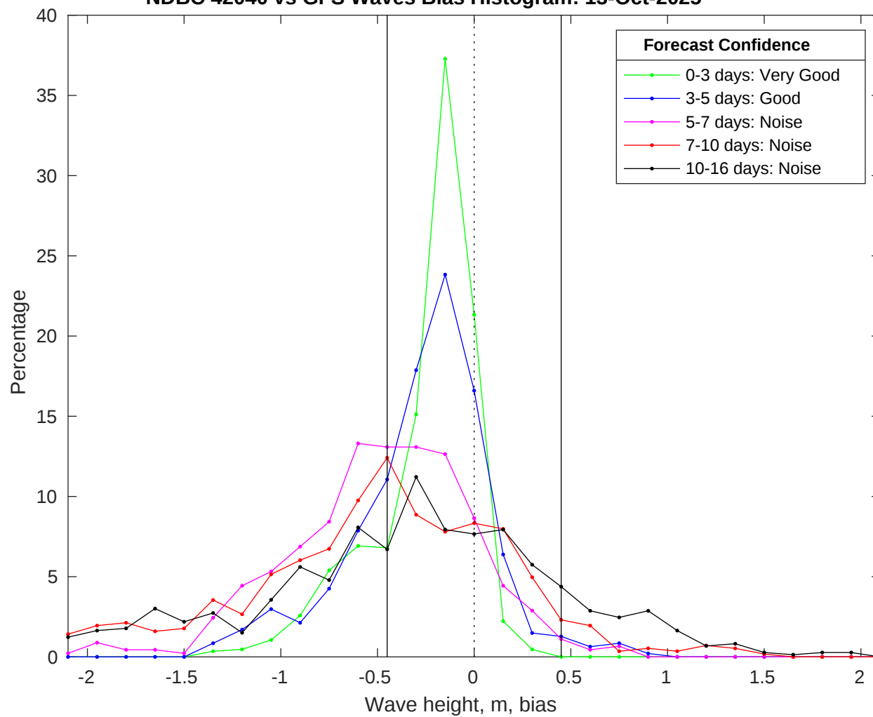
NDBC 42040 vs GFS Waves Bias Histogram: 13-Oct-2025
