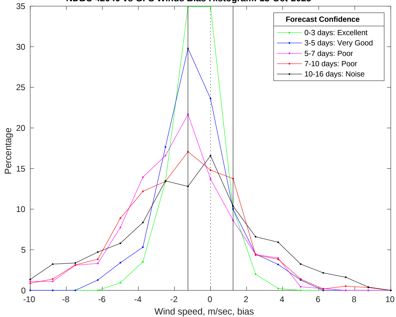
NDBC 42040 vs GFS Winds Bias Histogram: 13-Oct-2025
