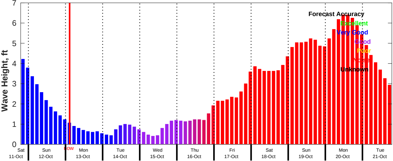
CMEMS Wave Forecast for NDBC 42040 from 11-Oct-2025 19:00:00 to 21-Oct-2025 19:00:00
