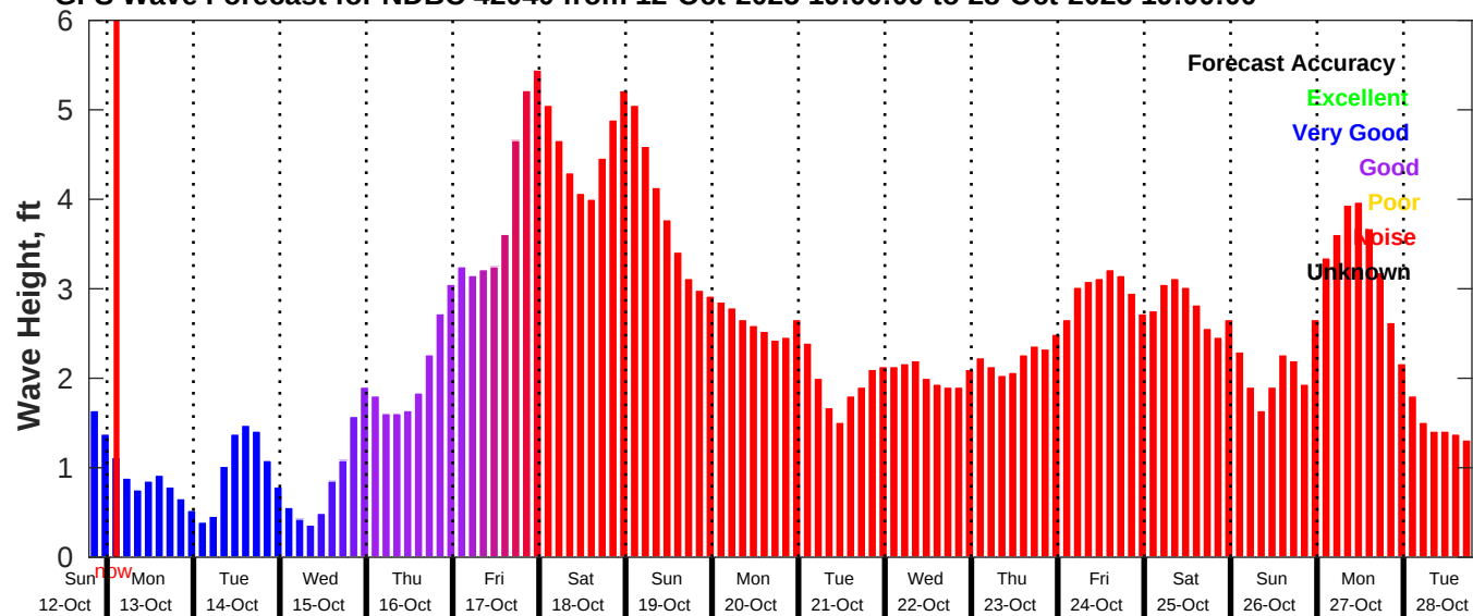
GFS Wave Forecast for NDBC 42040 from 12-Oct-2025 19:00:00 to 28-Oct-2025 19:00:00
