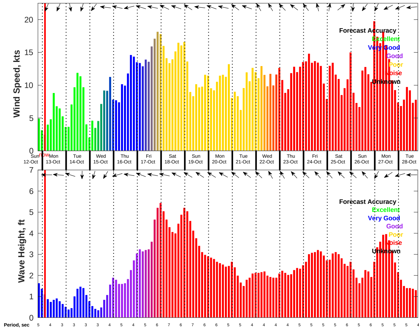
Wind & Wave Forecast for NDBC 42040 from 12-Oct-2025 19:00:00 to 28-Oct-2025 19:00:00
