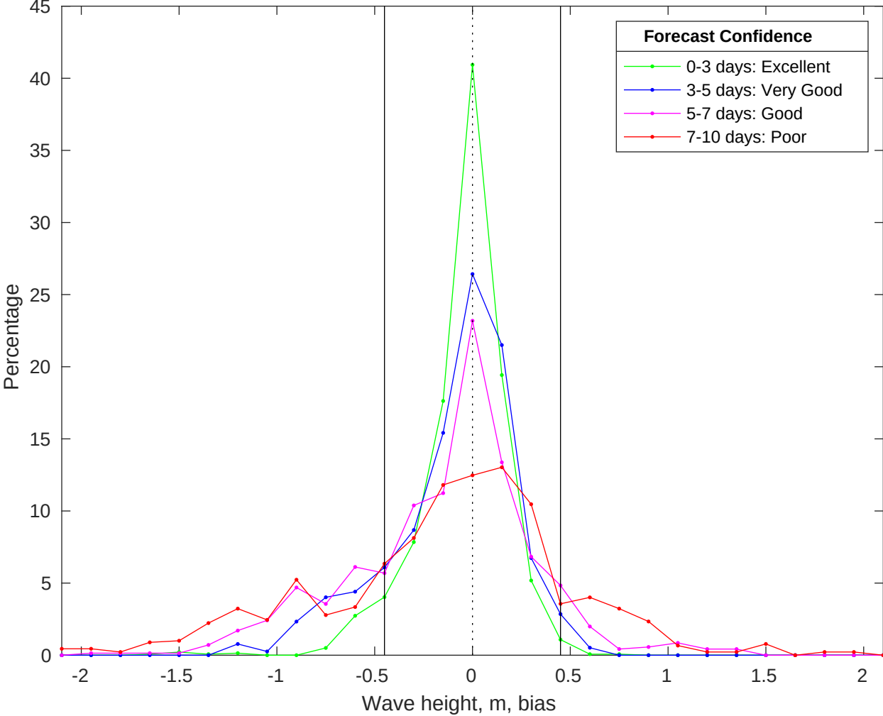
NDBC 44008 vs CMEMS Waves Bias Histogram: 13-Oct-2025
