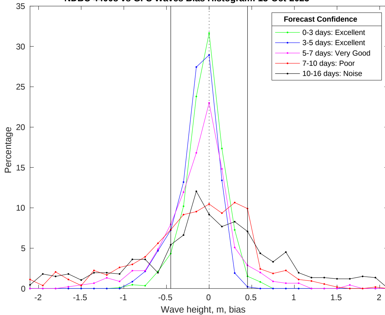
NDBC 44008 vs GFS Waves Bias Histogram: 13-Oct-2025
