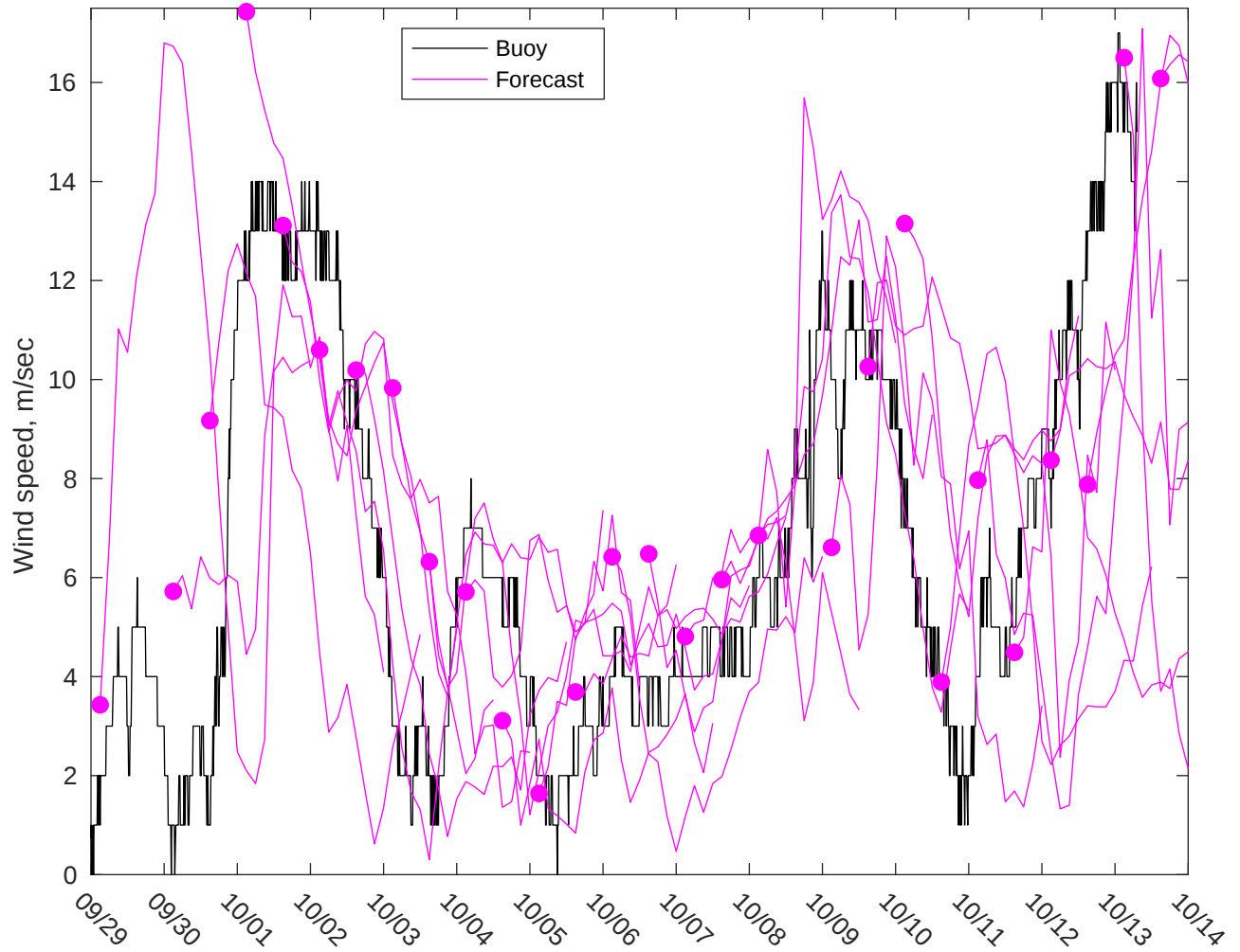
NDBC 44008 vs GFS Winds: 7 to 10 day forecast
