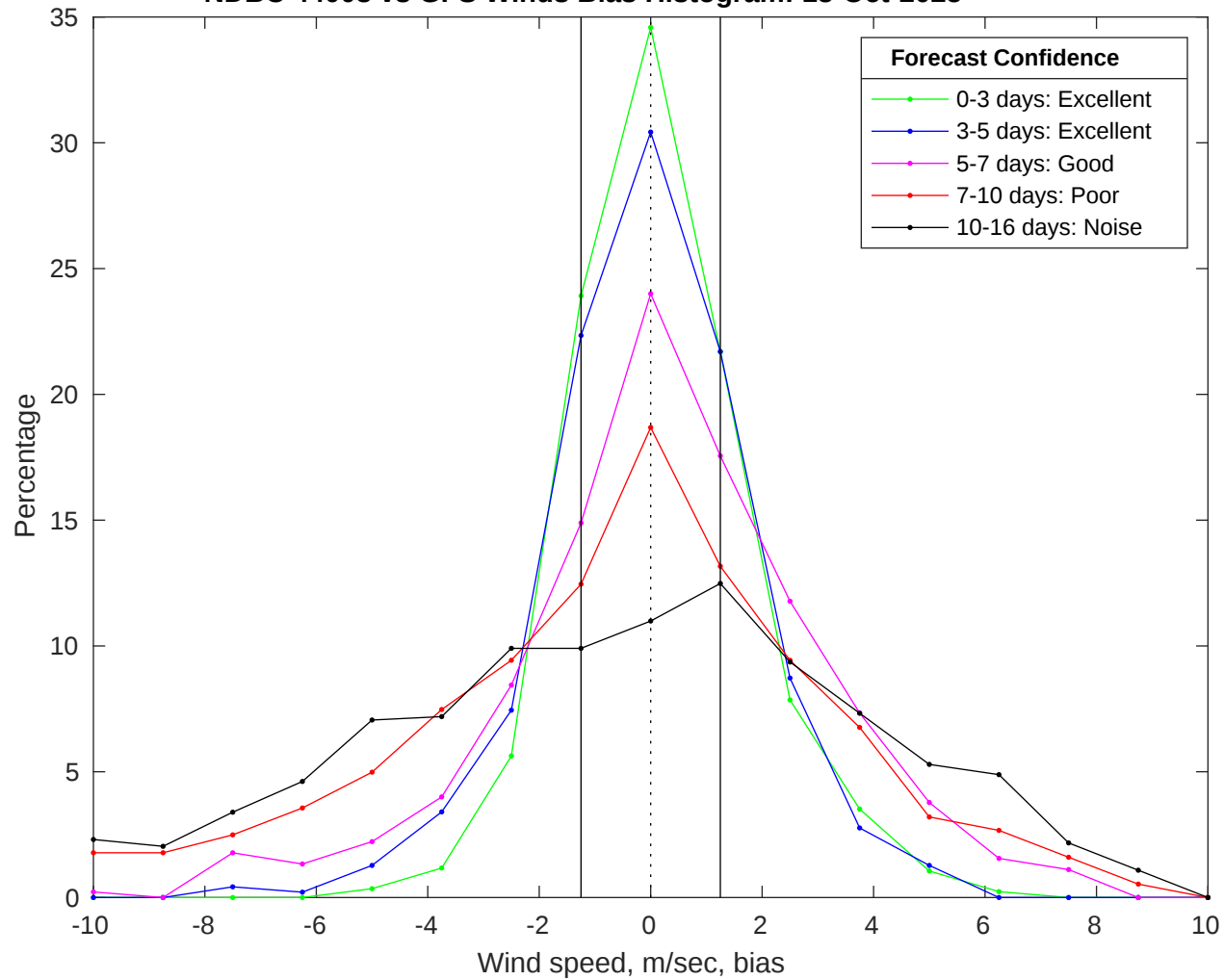
NDBC 44008 vs GFS Winds Bias Histogram: 13-Oct-2025
