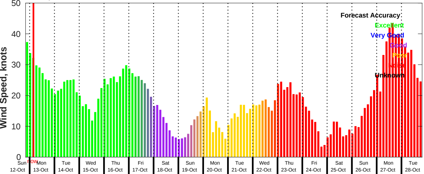
GFS Wind Speed Forecast for NDBC 44008 from 12-Oct-2025 20:00:00 to 28-Oct-2025 20:00:00
